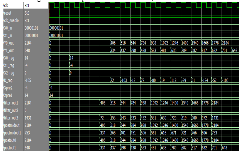
Fig. 8: Simulation of Modified Two Parallel FIR Filter Using Direct Multiplication
