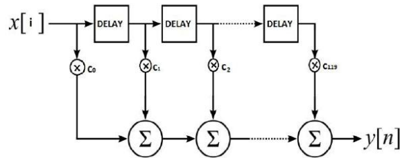
Fig. 1: FIR filter
