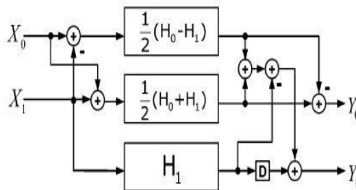
Fig. 4: Proposed Two Parallel FIR Filter using LUT less DA
