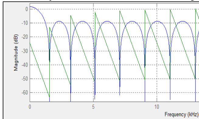
Fig. 6: Frequency and Phase Response
