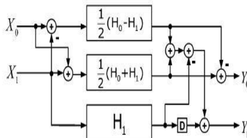
Fig. 3: Modified Two Parallel FIR Filter
