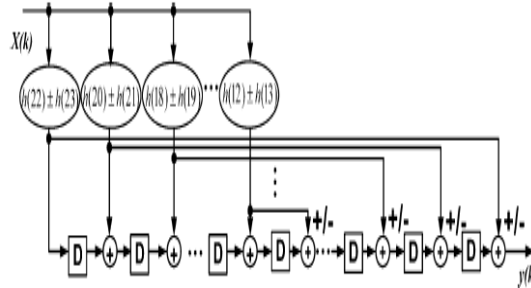
Fig. 5: Sub filter Block Implementation with Symmetric Coefficients
