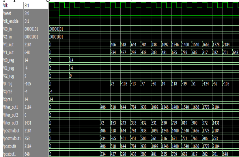
Fig. 9: Simulation of Proposed Two Parallel FIR Filter Using LUT less DA
