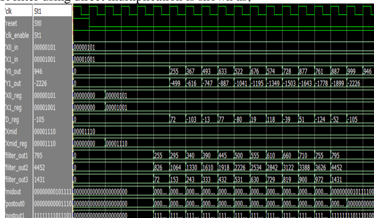
Fig. 7: Simulation of Traditional Two Parallel FIR Filter Using Direct Multiplication
