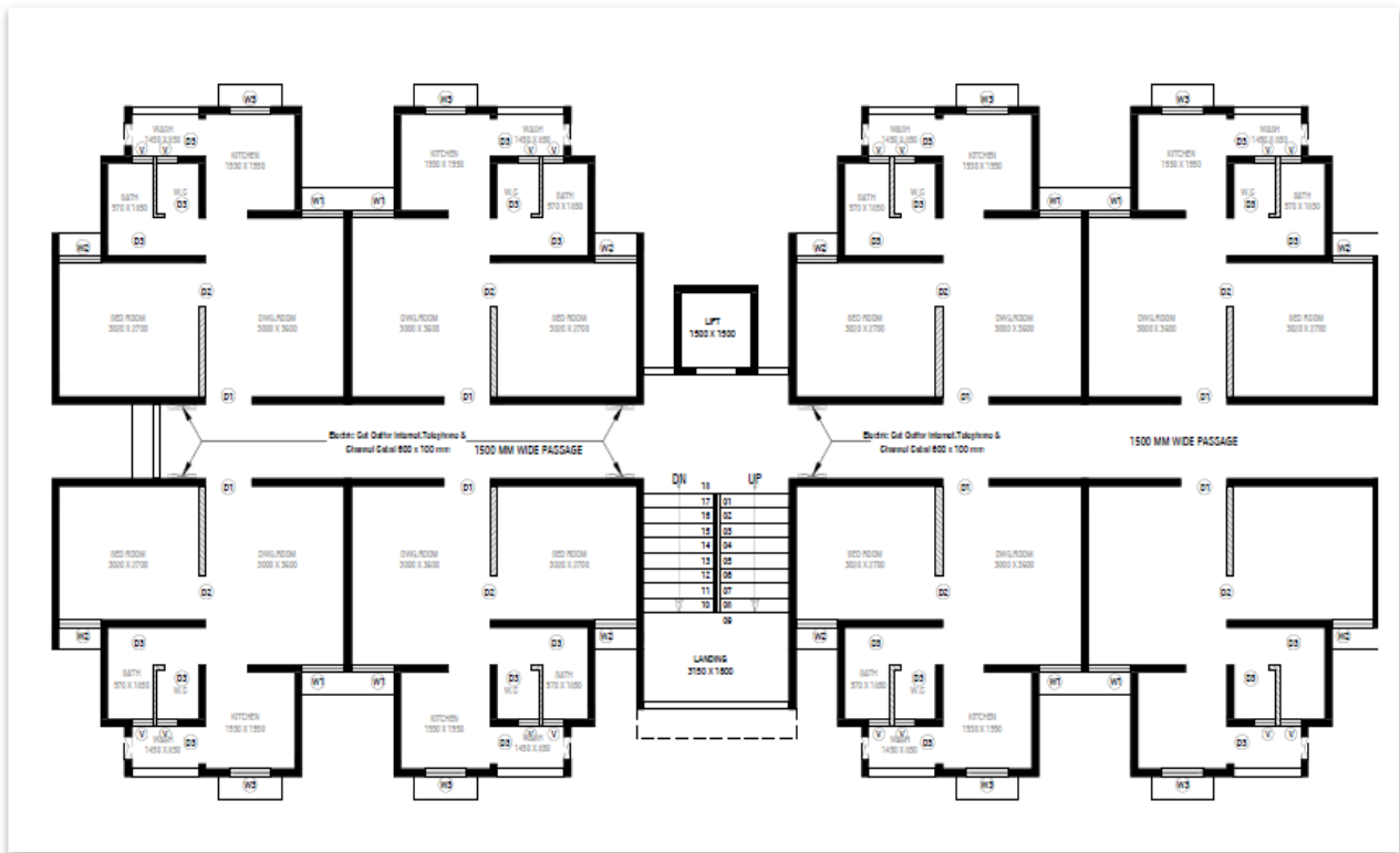
Fig. 1: Building Plan
