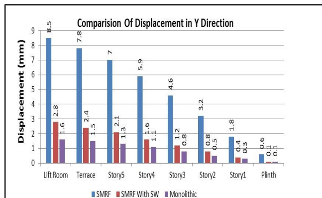
Fig. 3: Comparison of Displacement in Y Direction
