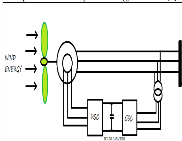
Fig. 1: DFIG based WECS
