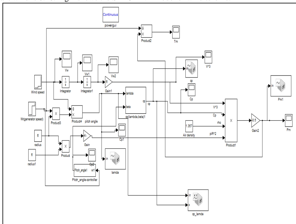
Fig. 2: Simulink model of Wind Turbine
