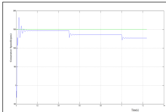
Fig. 9: Generator Speed
