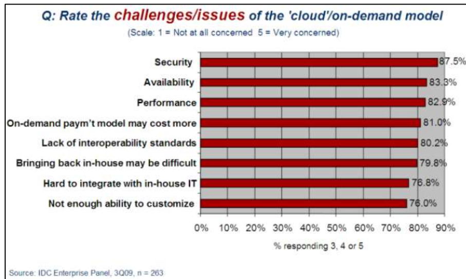
Fig. 1: Security issue
