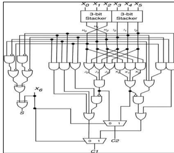
Fig. 3: 7:3 Counters based on symmetric stacking
