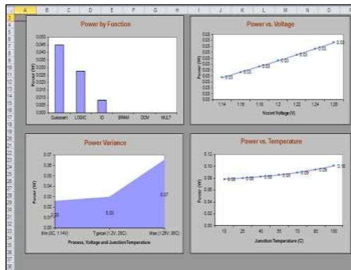
Fig. 8: Power New Full Adder (NFA) Counters
