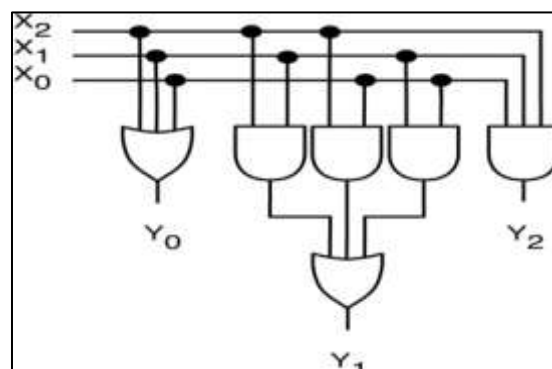
Fig. 2: Three-bit stacker circuit
