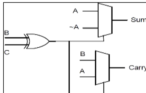
Fig. 4: Proposed Full Adders
