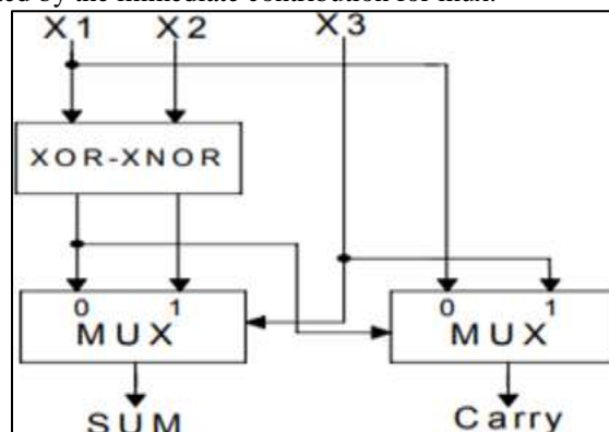
Fig. 1: Conventional counter
