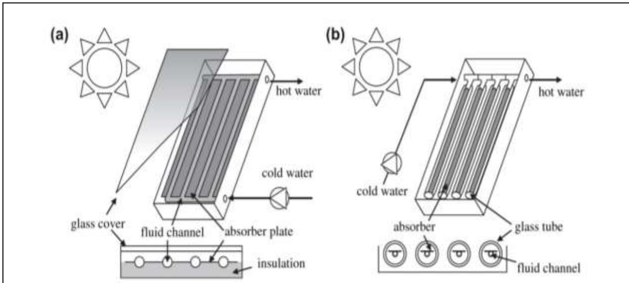
Fig. 1: Schematic diagrams of non-concentrating solar collectors (a) flat plate type and (b) evacuated type
