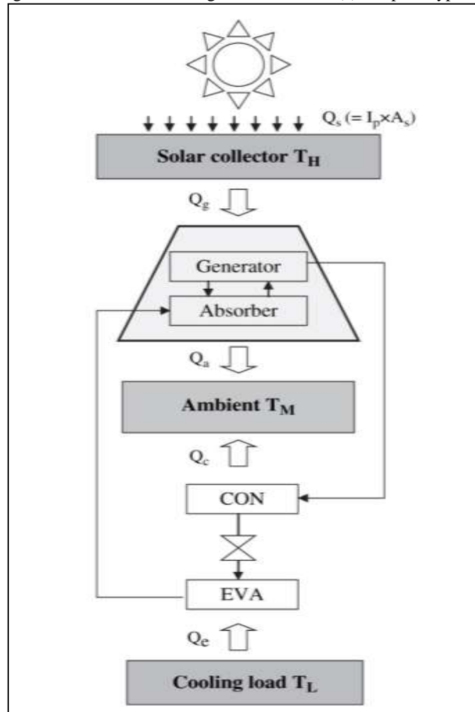
Fig. 2: Solar absorption refrigeration system
