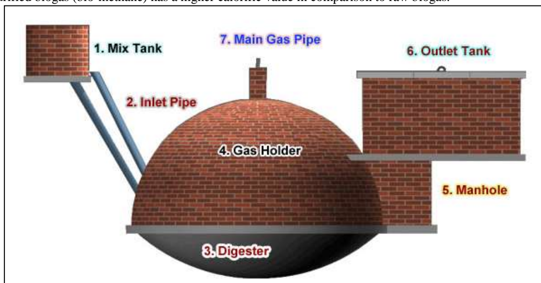
Fig. 4: Biogas Plant
