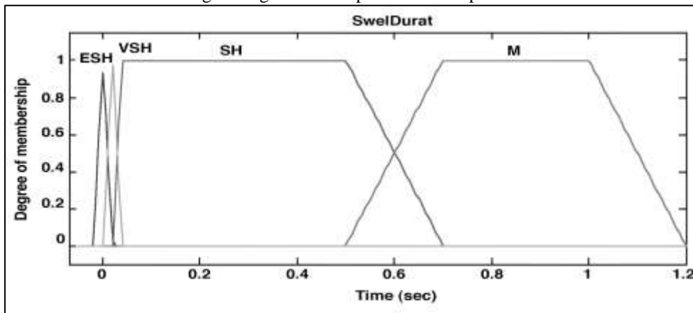
Fig. 5: Swell duration input membership functions
