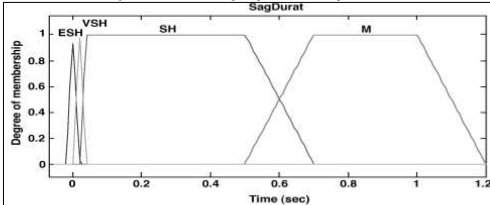
Fig. 4: Sag duration input membership function
