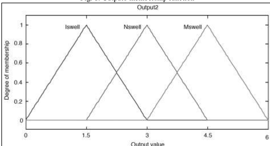
Fig. 9: Output2 membership function
