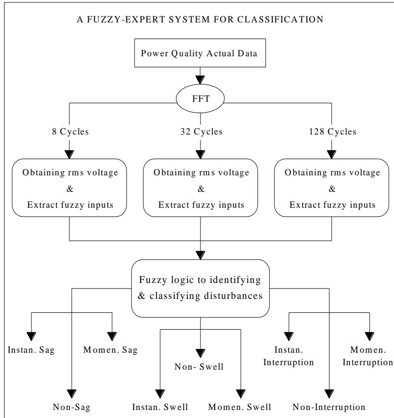
Fig. 3: Design of the proposed fuzzy-expert system
