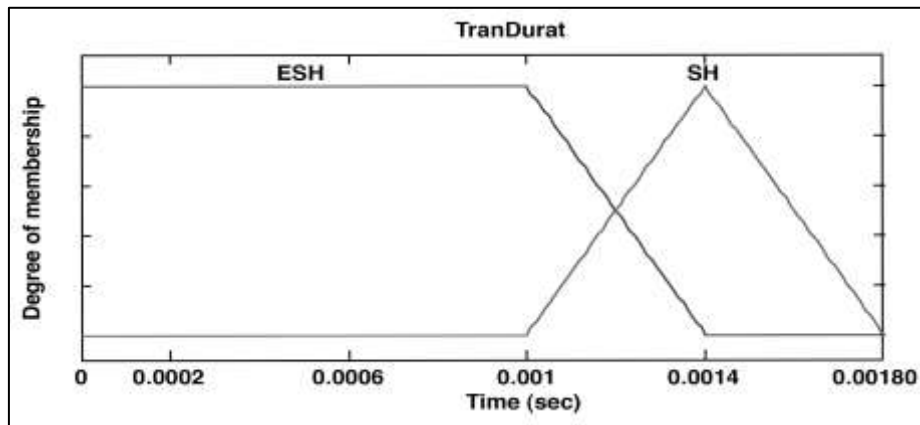
Fig. 6: Transient duration input membership functions
