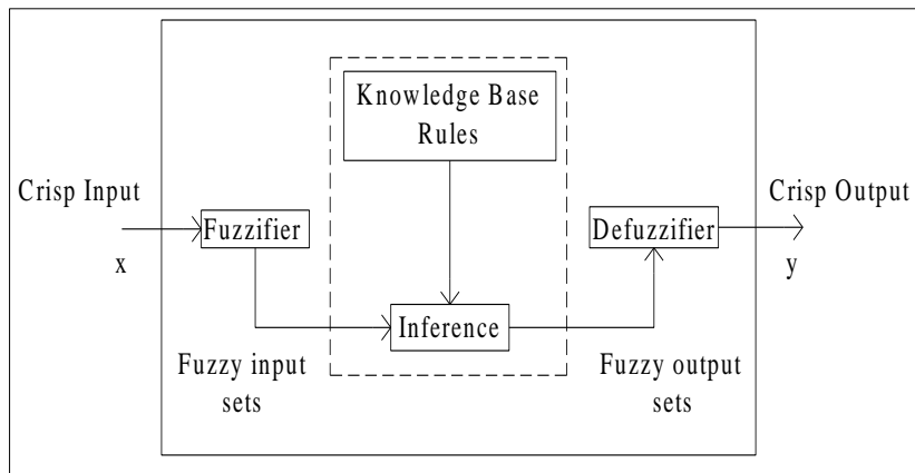
Fig. 2: Fuzzy Controller Architecture
