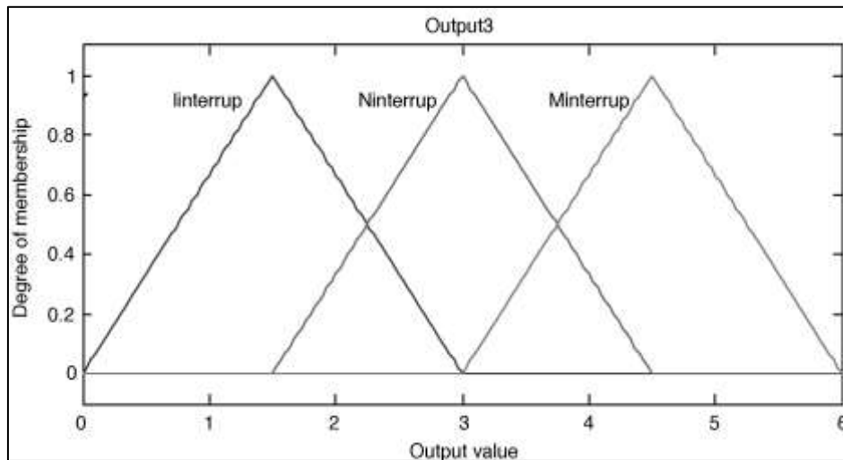
Fig. 10: Output3 membership function
