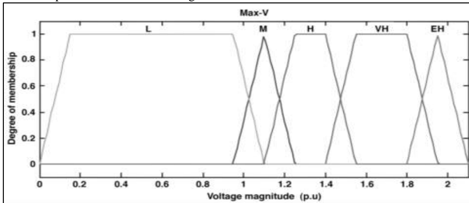
Fig. 3: Maximum voltage input membership function
