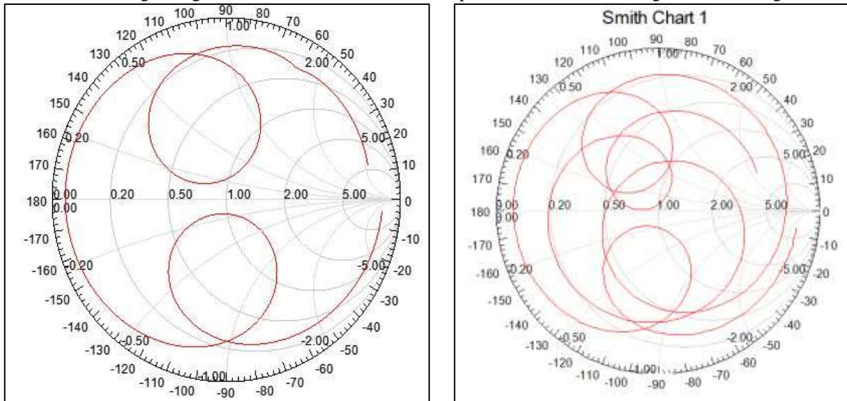
Fig. 6: Smith chart of proposed antenna-1 and antenna-2
