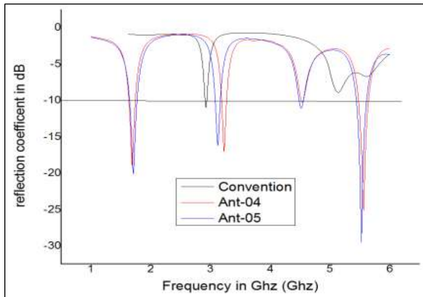
Figure 4: Reflection coefficient of conventional and DGS embedded antennas.
