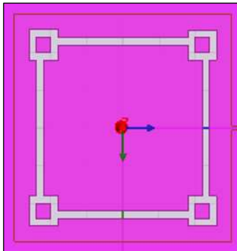
Fig. 2: DGS of Antenna-1.
