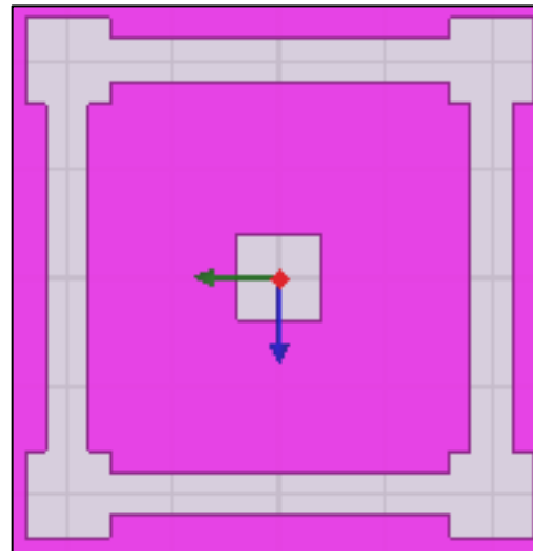
Fig. 3: DGS of Antenna-2.
