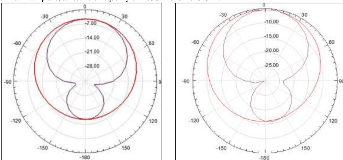
Fig. 5: The Radiation pattern of the designed antenna-1 and antenna-2.
